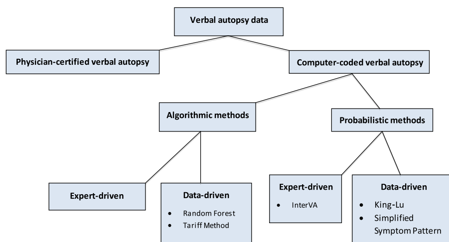
Figure 1 Classification of verbal autopsy interpretation methods.
